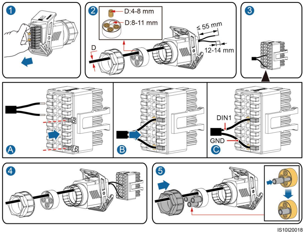
Figure 5-32 Installera kabeln
