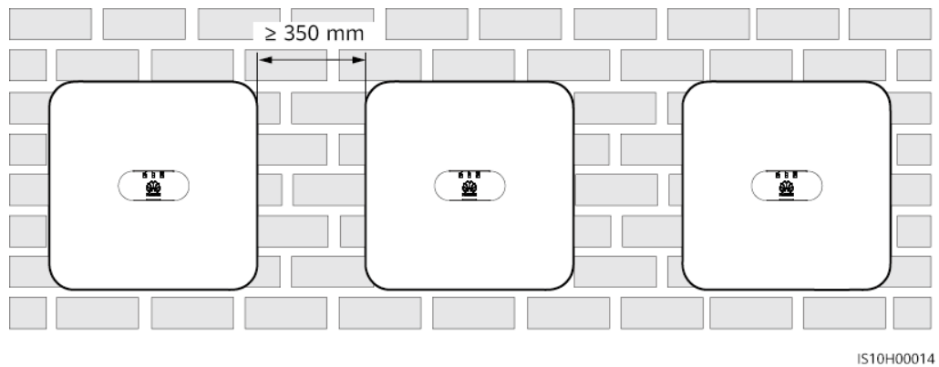
Figure 4-3 Horisontell installation (rekommenderas)
