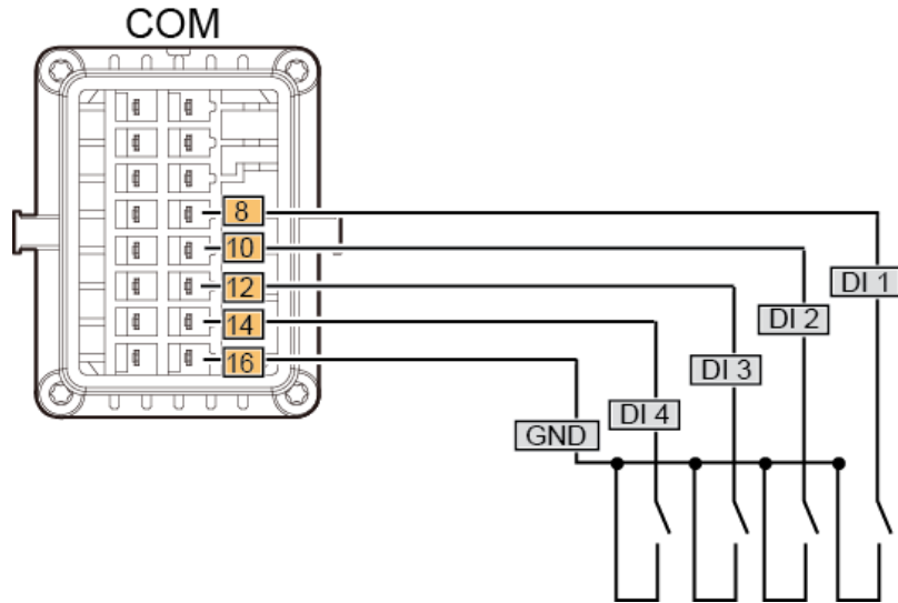
Figure 5-29 Kabelanslutning
