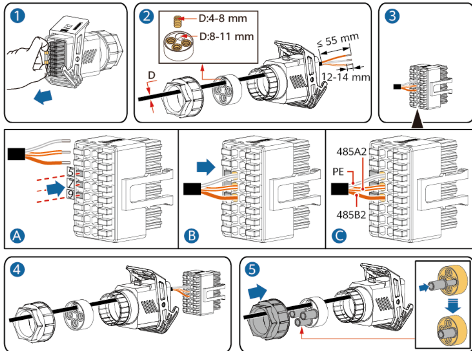
Figure 5-25 Installera kabeln
